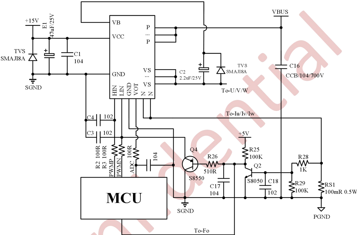
Fig.8 Typical Application Connection NSH706PQ
