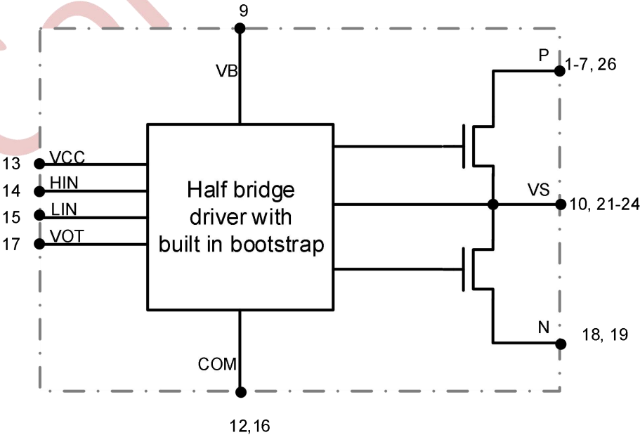
Fig.1 Internal Electrical Schematic
