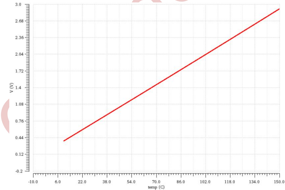
Fig. 4 Curves of HVIC Temperature detection—voltage curve
